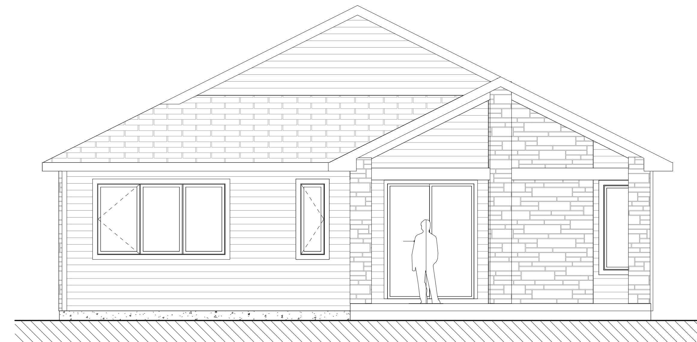
REAR ELEVATION
