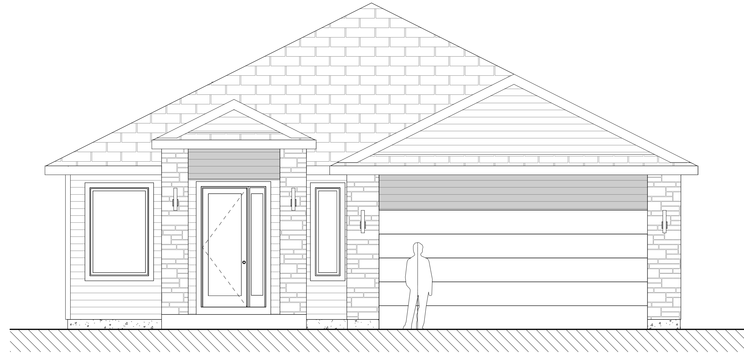
FRONT ELEVATION
