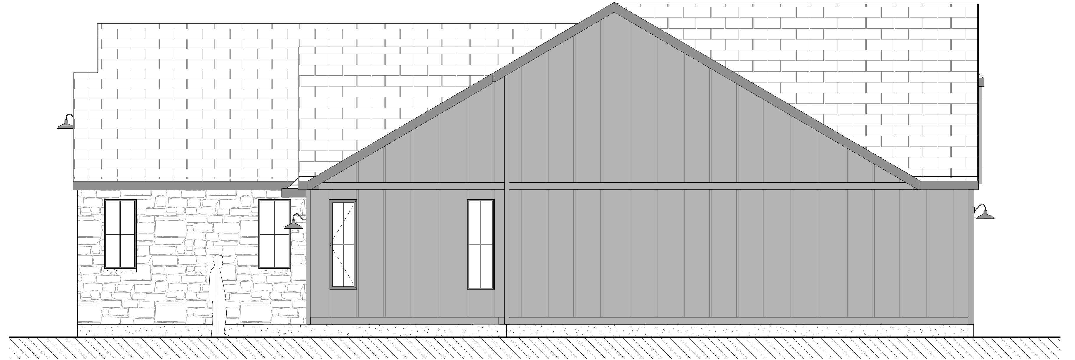
LEFT ELEVATION
