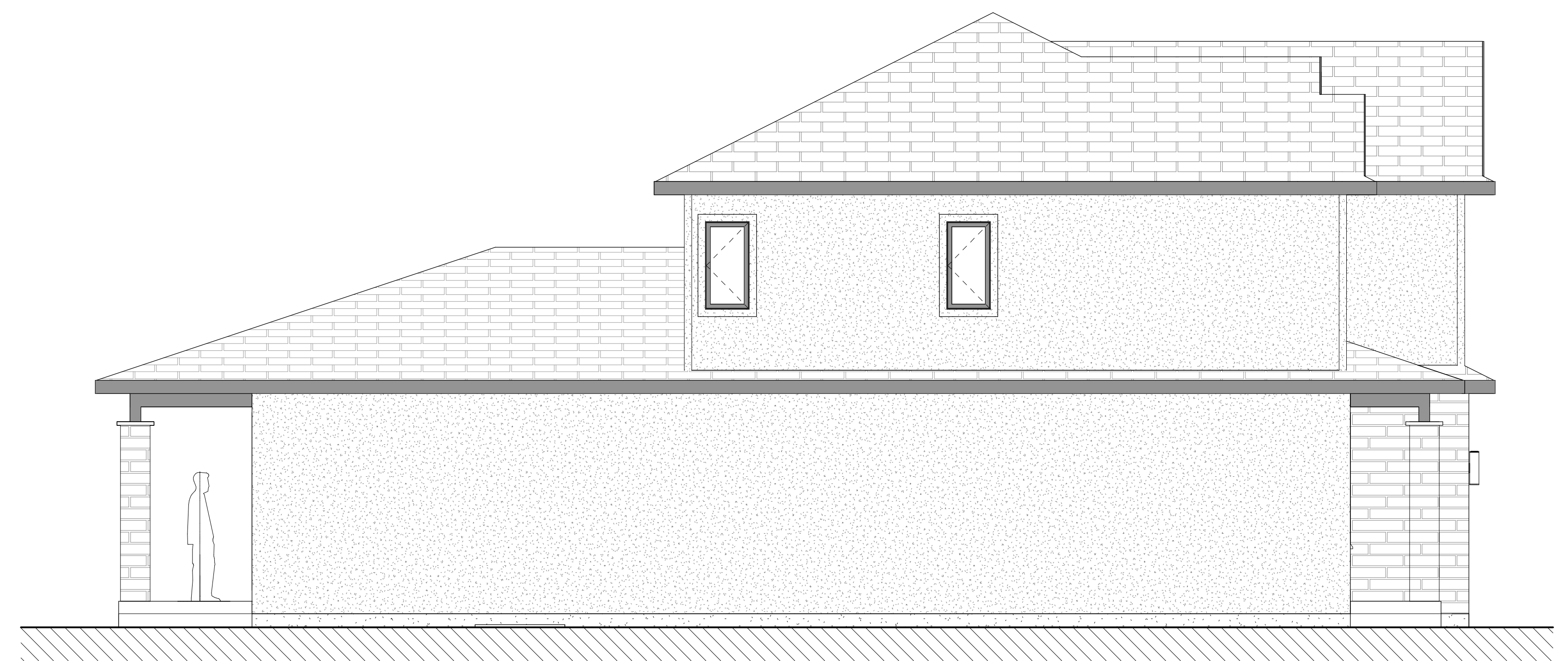
LEFT ELEVATION
