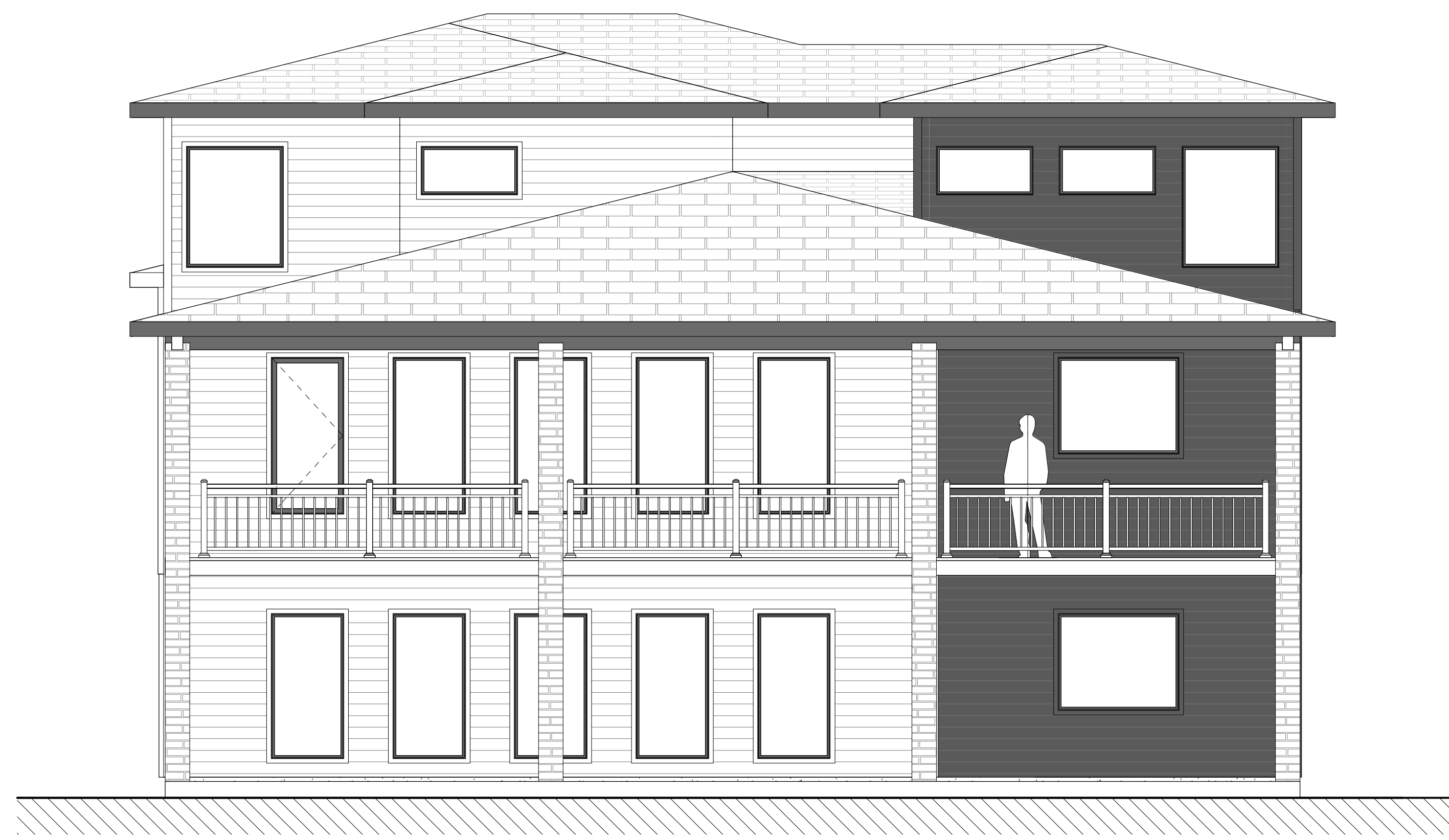
REAR ELEVATION
