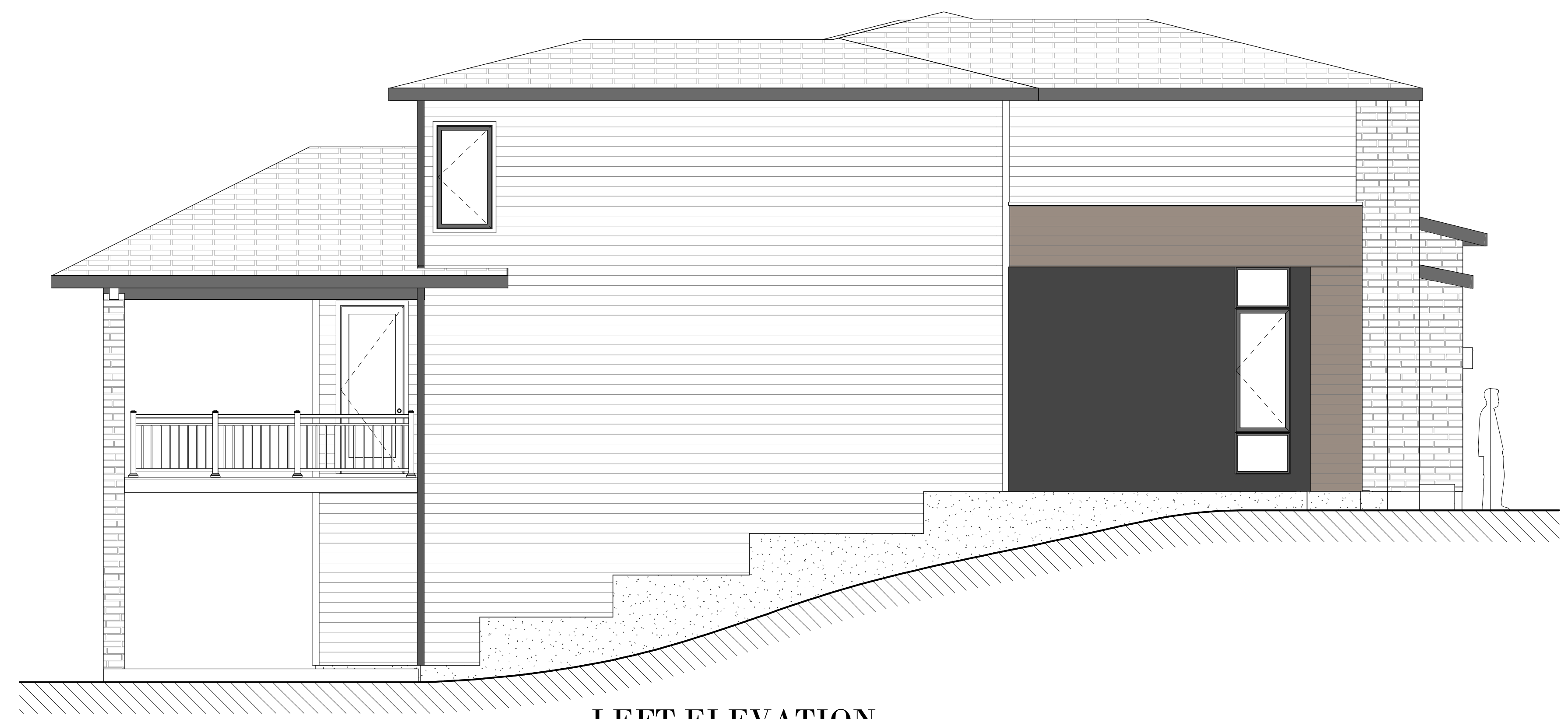
LEFT ELEVATION
